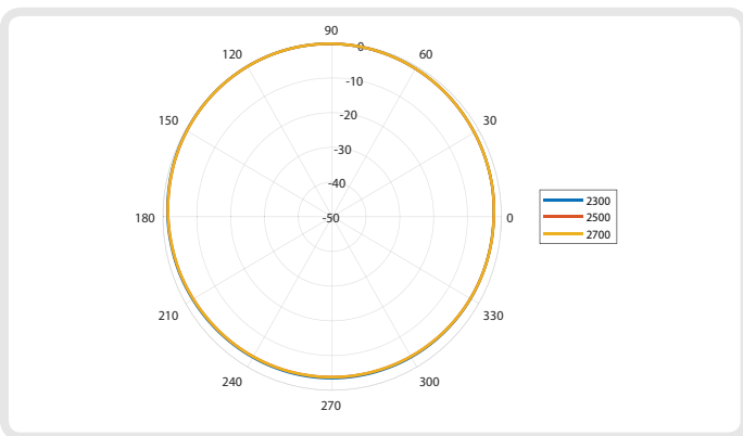
Azimuth: 2300 - 2700 MHz
