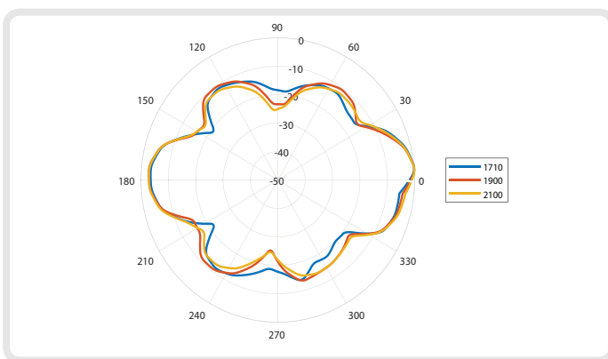
Elevation: 1710 - 2100 MHz
